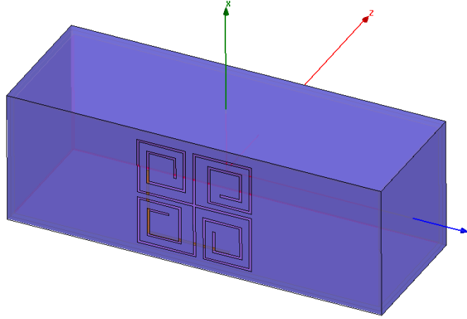
Fig. 5.8: Spiral slot antenna on 3U CubeSat.
