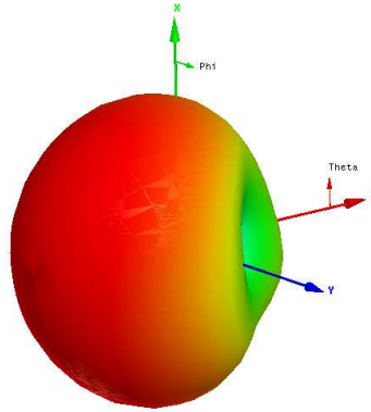
Fig. 5.5: Radiation gain of the rectangular slot antenna.
