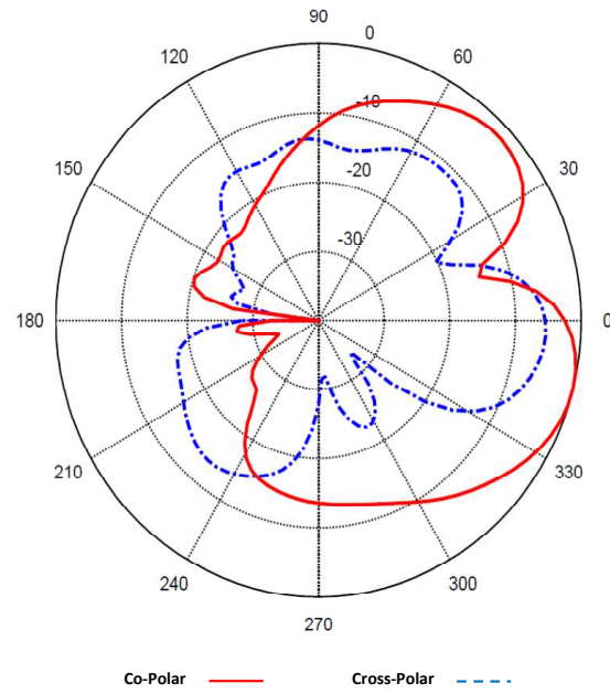
Fig. 3.21: Measured co-polar and cross-polar components of the radiation pattern of the array in E-plane at 2.56\text{ GHz} .
