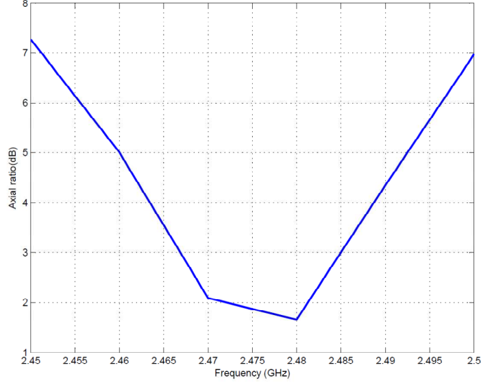
Fig. 3.14: Measured AR of the fabricated cross slot antenna.
