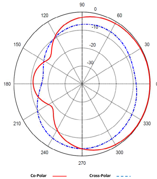
Fig. 3.22: Measured co-polar and cross-polar components of the radiation pattern of the array in H-plane at 2.56\text{ GHz} .
