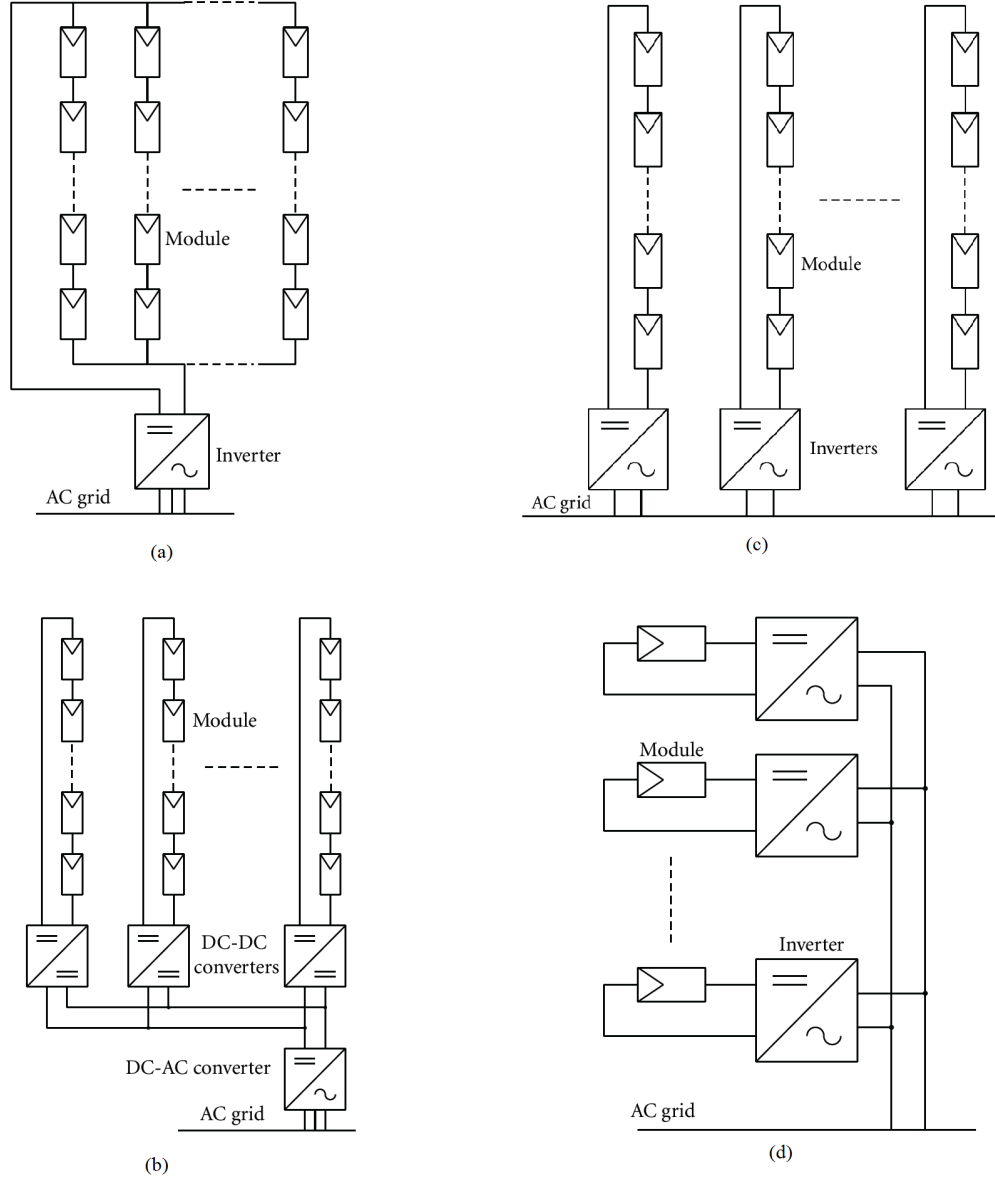
Fig. 1.5: Different commercial configurations of grid-connected PV systems: (a) central plant inverter, (b) multiple string DC-DC converter, (c) multiple string inverter, and (d) module integrated inverter.
