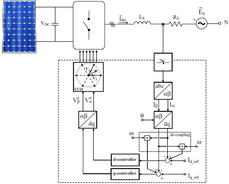
Fig. 3.1: Three-phase synchronous frame current controller scheme.
