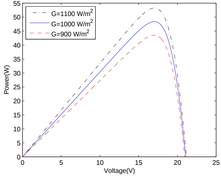
Fig. 4.13: P-V chart of considered PV model for different sun irradiation (temperature = 25^\circ\text{C} ).
