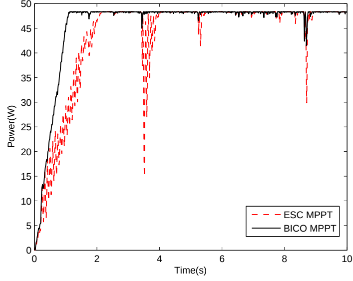
Fig. 4.16: Performance of BICO MPPT and ESC MPPT in the presence of a white noise with \text{PSD} = 0.04\text{W}/\text{Hz} .
