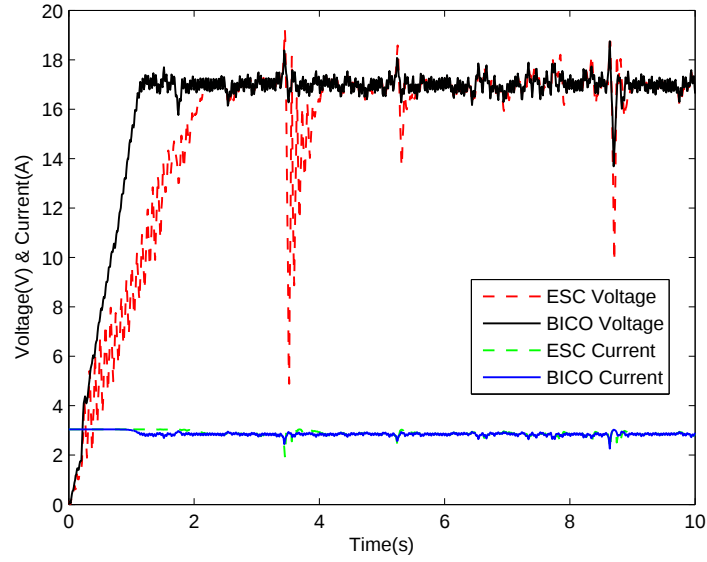
Fig. 4.17: Voltage and current tracking of BICO MPPT and ESC MPPT in the presence of a white noise with \text{PSD} = 0.04\text{W}/\text{Hz} .
