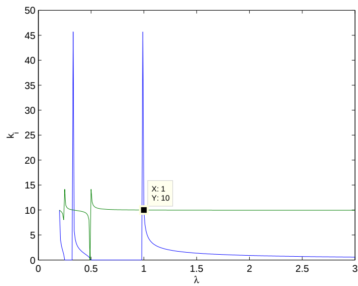
Fig. 5.19: Graphical method of finding k_i and \lambda for FO-[PI].
